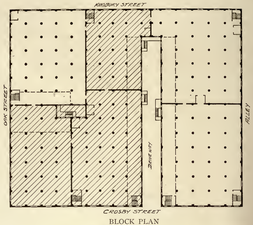
BLOCK PLAN
